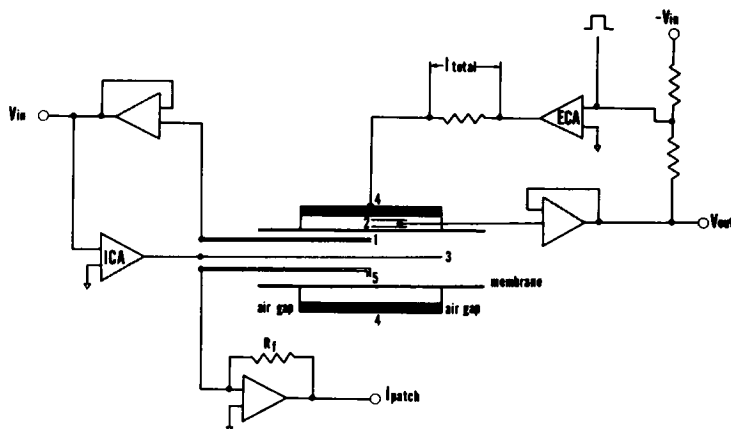
FIGURE 1 Voltage clamp and current recording circuit. The numbers in the diagram refer to the following electrodes: 1, internal voltage pipette; 2, external voltage electrode; 3, internal platinized-platinum axial current passing wire; 4, external platinized-platinum electrodes; and 5, L-shaped patch pipette. The large external electrodes (4) were 15 mm long and extended the entire length of the axon between the air gaps, so I_{total} was recorded from this length of axon.
